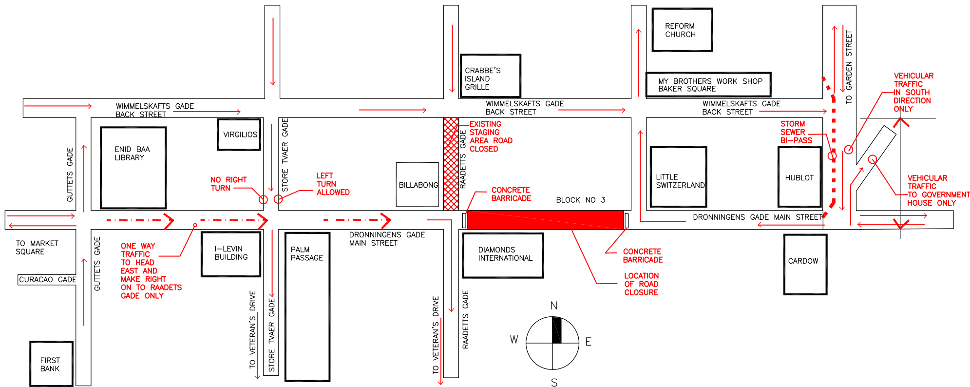
MAINTENANCE OF TRAFFIC PLAN MAIN STREET ENHANCEMENT PROJECT
